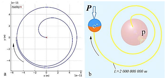
Figure 1. Electron birth and spiral capture into the first Bohr orbit during neutron \beta -decay.
